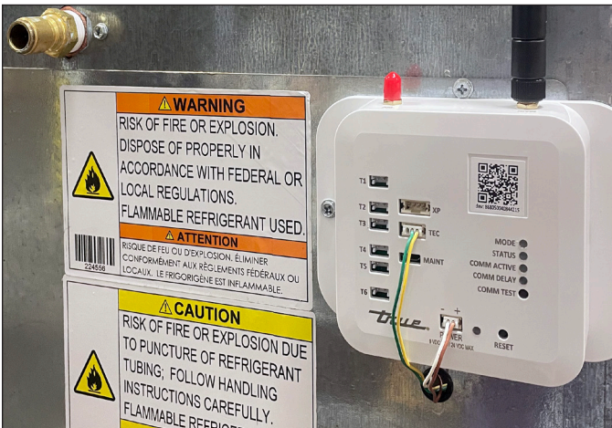
Fig. 2. Wire harness connected to modem. Green/Yellow to TEC; Brown/White to POWER.
